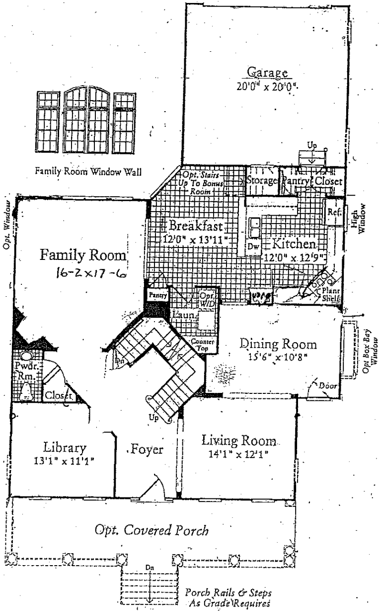
Standard First Floor Plan
